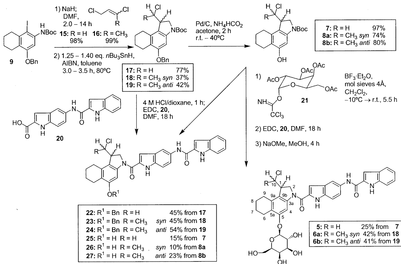
Scheme 5. Preparation of the seco -CCI derivatives for the biological tests; AIBN = \alpha,\alpha' -Azobisisobutyronitrile, EDC = N -ethyl- N' -(3-dimethylaminopropyl)carbodiimide hydrochloride
