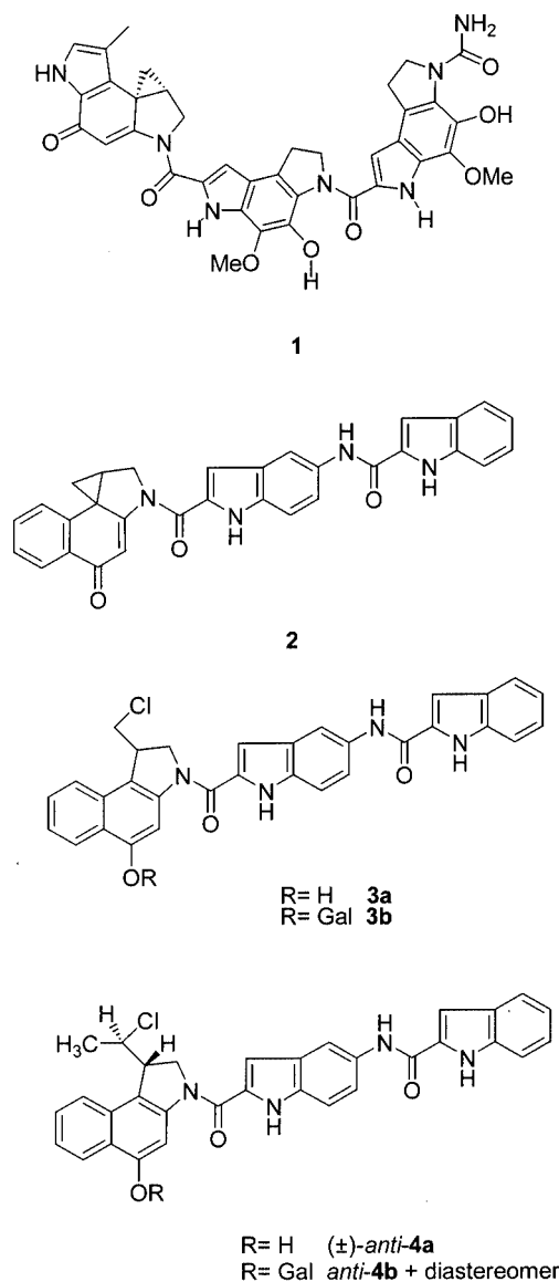
Scheme 1. Structure of (+)-CC-1065 ( 1 ) and the analogues CBI ( 2 ), seco -CBI 3a , and methyl- seco -CBI 4a , and their prodrugs 3b and 4b
