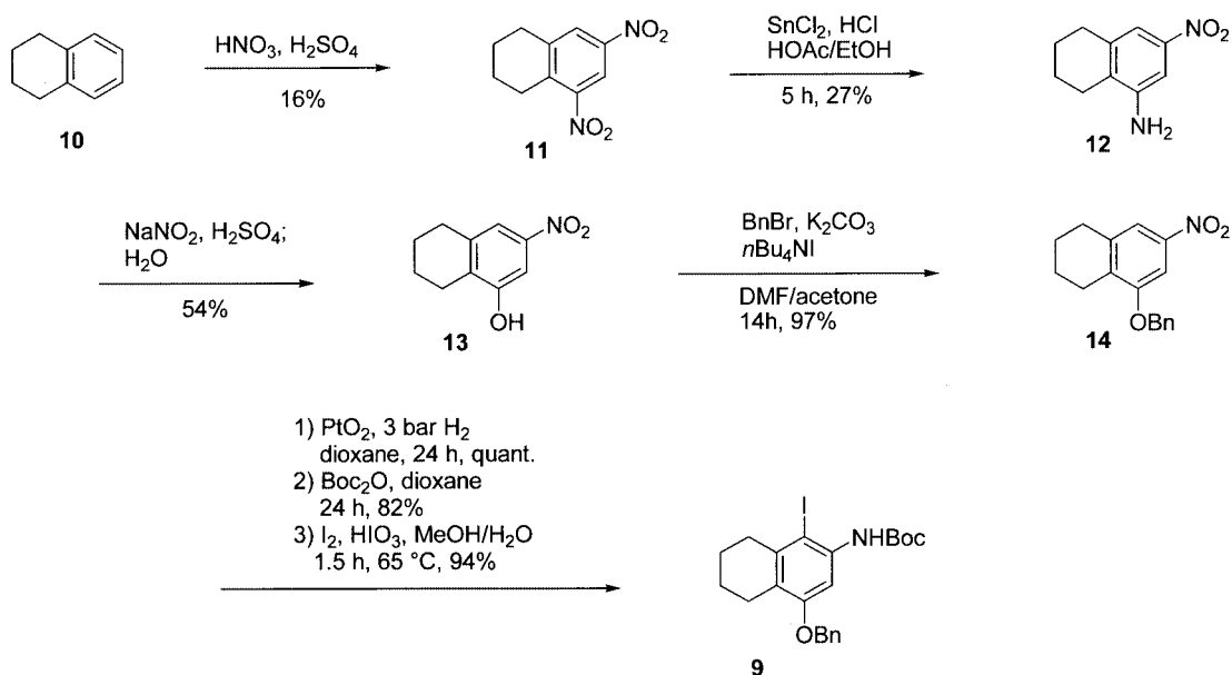
Scheme 4. Synthesis of the key intermediate 9
