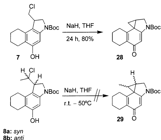
Scheme 6. Winstein cyclization of partially hydrogenated seco -CBI analogues
