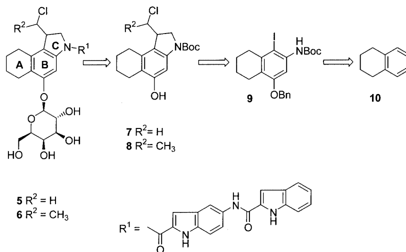
Scheme 3. Retrosynthesis of the novel partially hydrogenated prodrugs 5 and 6
