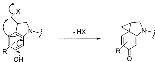
Scheme 2. Formation of the spirocyclopropylcyclohexadienone moiety of CC-1065 and its analogues by Winstein cyclization from the seco -compounds
